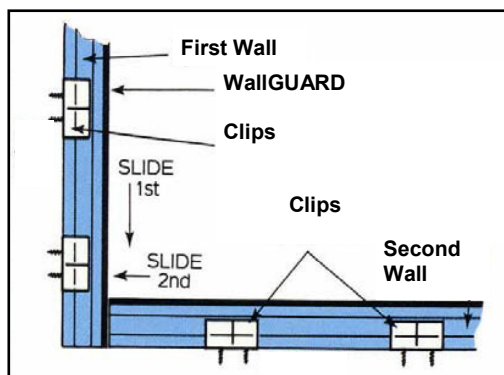
Horizontal Installation - Inside Corner Detail Top View
