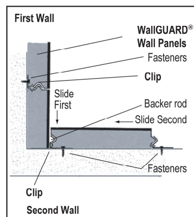
Vertical Installation - Inside Corner Detail Top View
