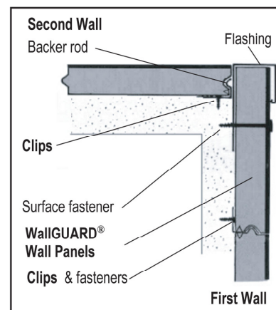
Vertical Installation - Outside Corner Detail Top View
