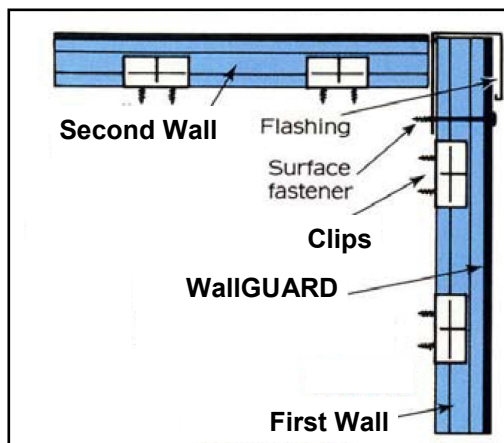
Horizontal Installation - Outside Corner Detail Top View
