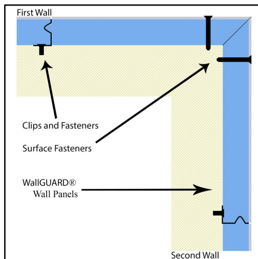
Mitered Corner Installation Detail Top View
